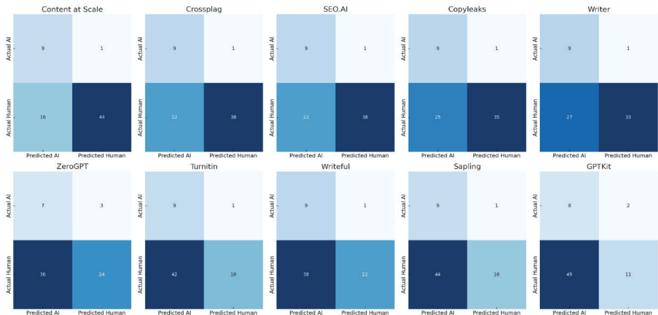
Figure 3. Confusion Matrices
