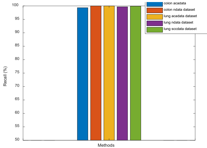
Figure 25. Recall Performance
