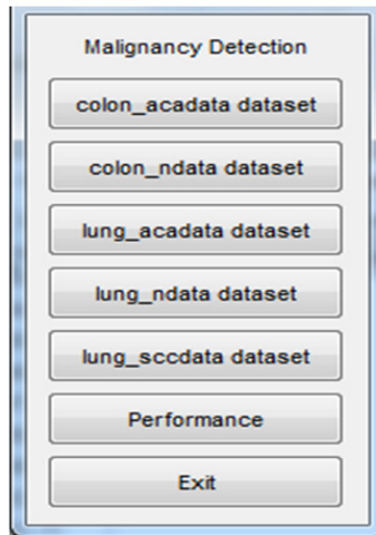
Figure 8. Main Menu
