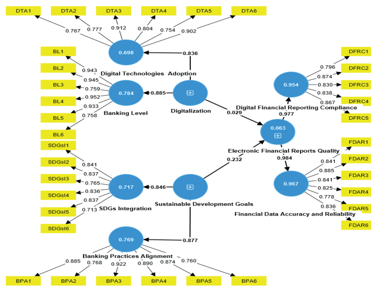
Figure 2. Measurement Model
